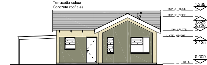
South Elevation
