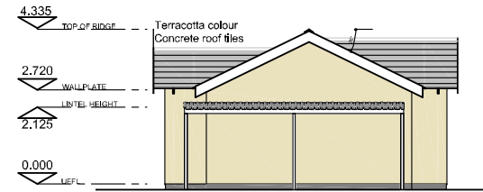
West Elevation
