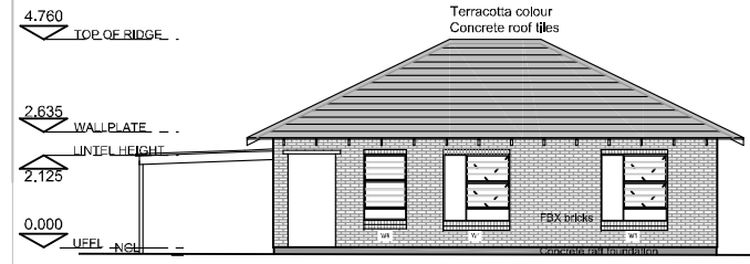
North Elevation
