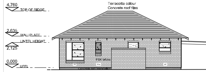
South Elevation
