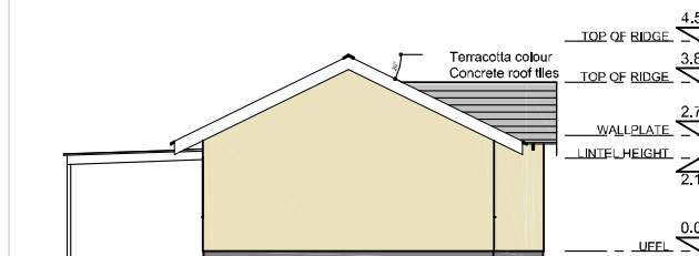
East Elevation
