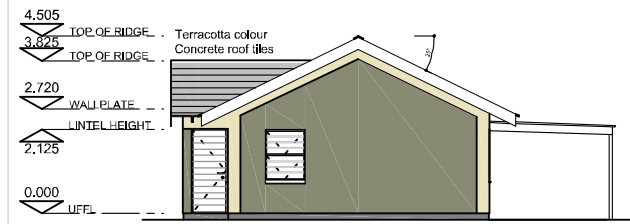
West Elevation
