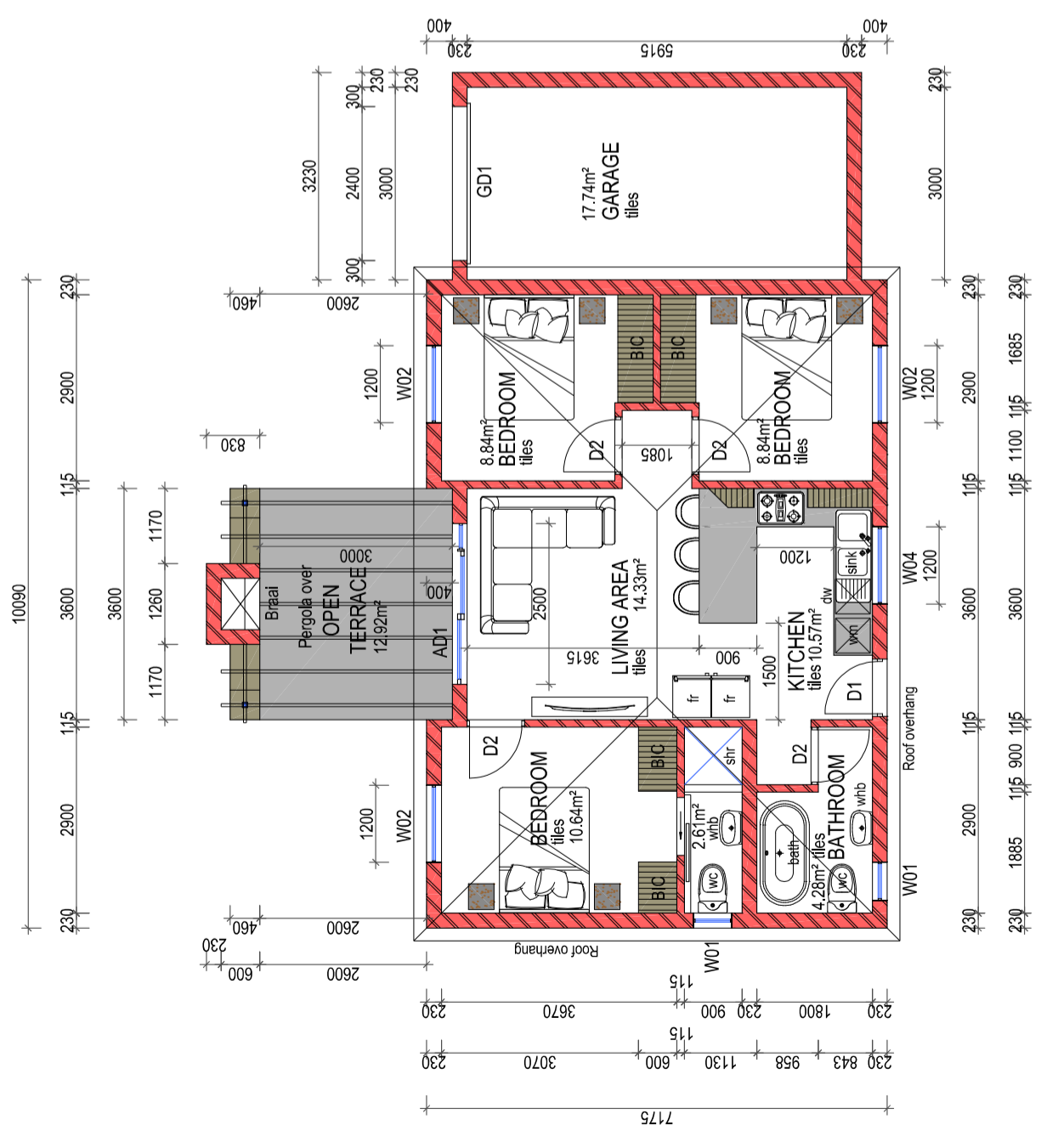
GROUND FLOOR PLAN UNIT B scale 1:100
