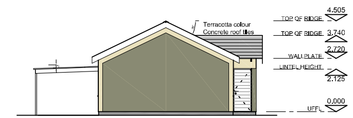
East Elevation
