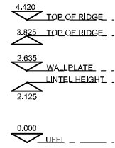
West Elevation
