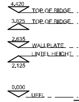
South Elevation
