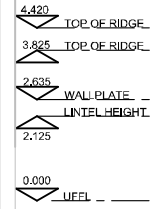
North Elevation
